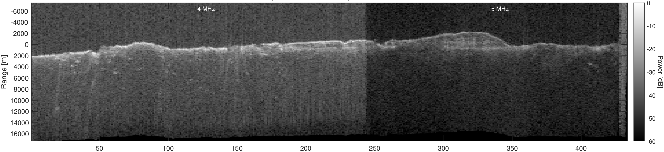
Orbit 21539, Optimized, Window, Depth-Corrected, Channel 2
