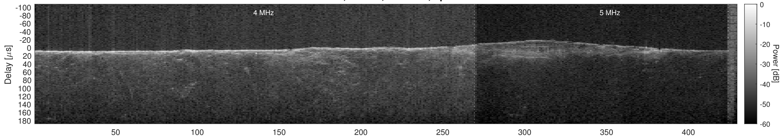
Orbit 21549, Cluttergram
