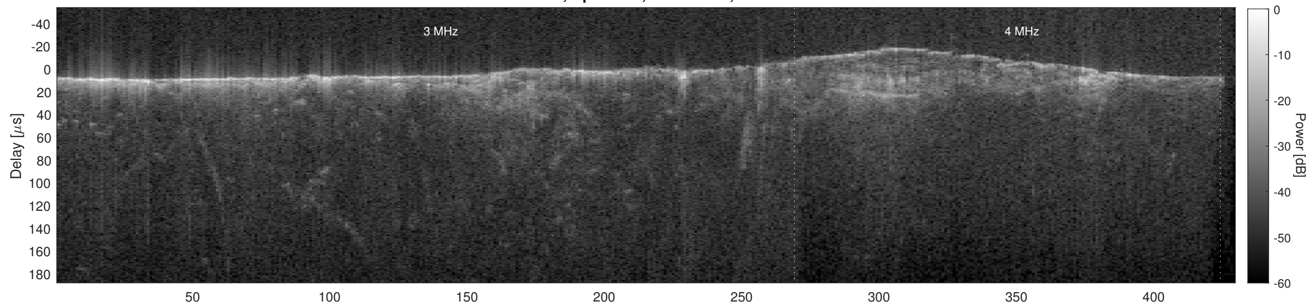
Orbit 21549, Cluttergram
