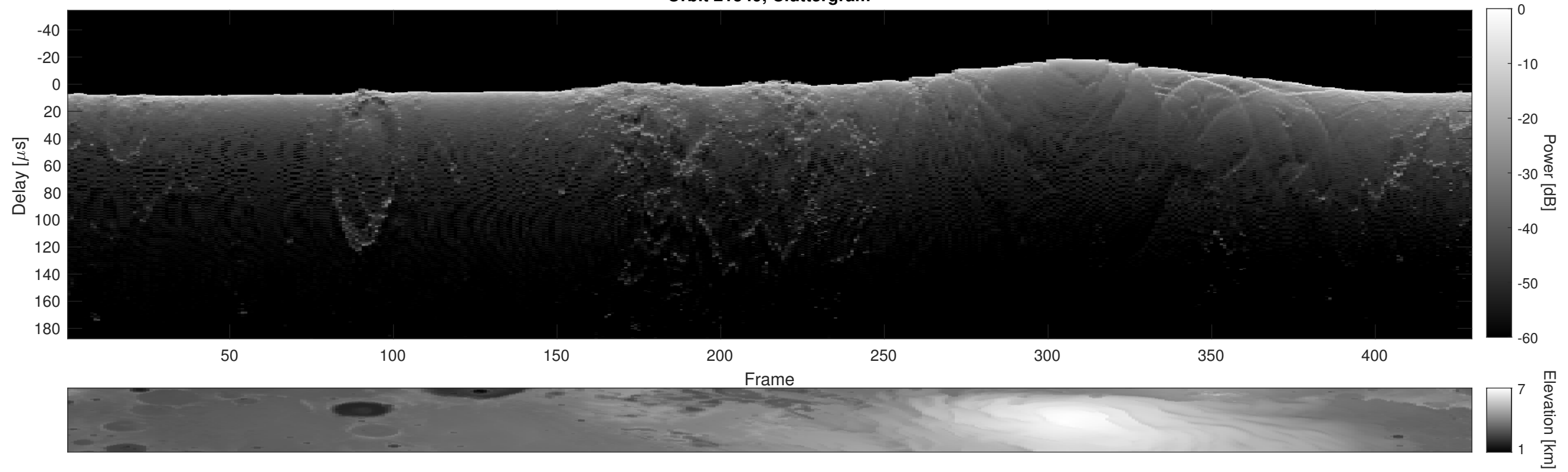
Orbit 21549, Cluttergram
