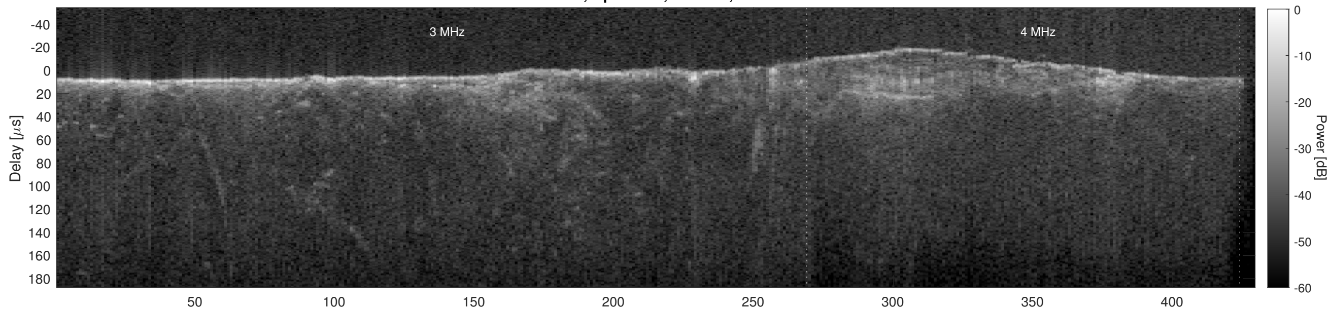
Orbit 21549, Cluttergram
