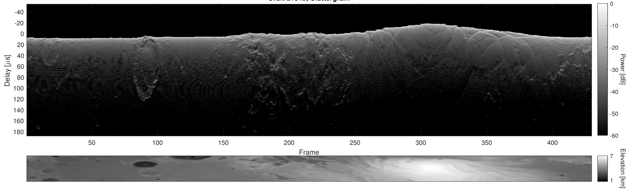
Orbit 21549, Cluttergram
