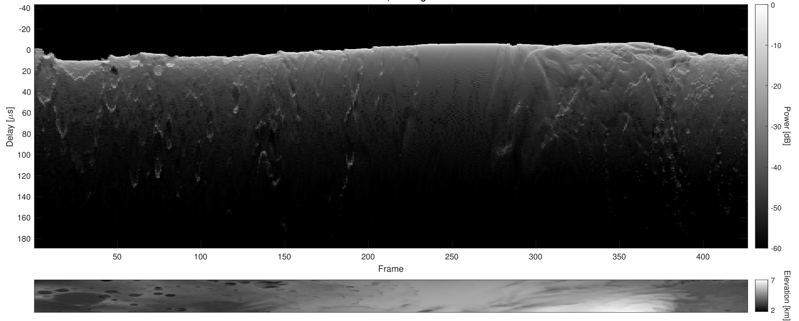
Orbit 21557, Cluttergram
