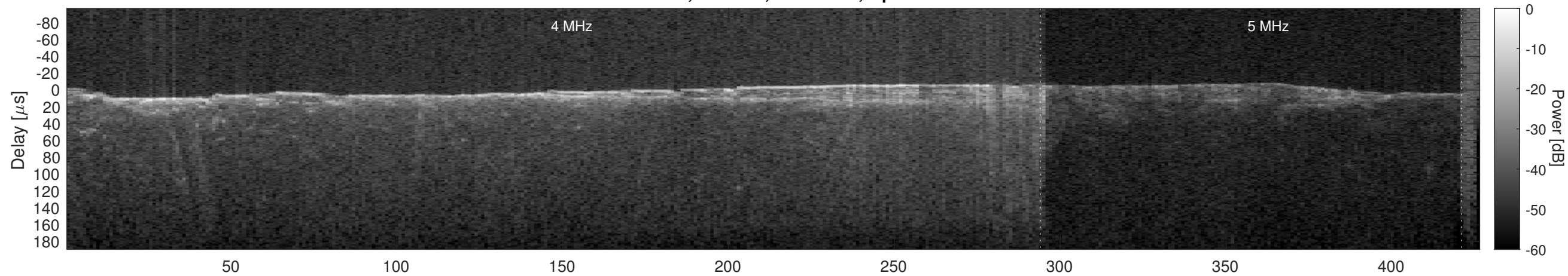
Orbit 21557, Cluttergram
