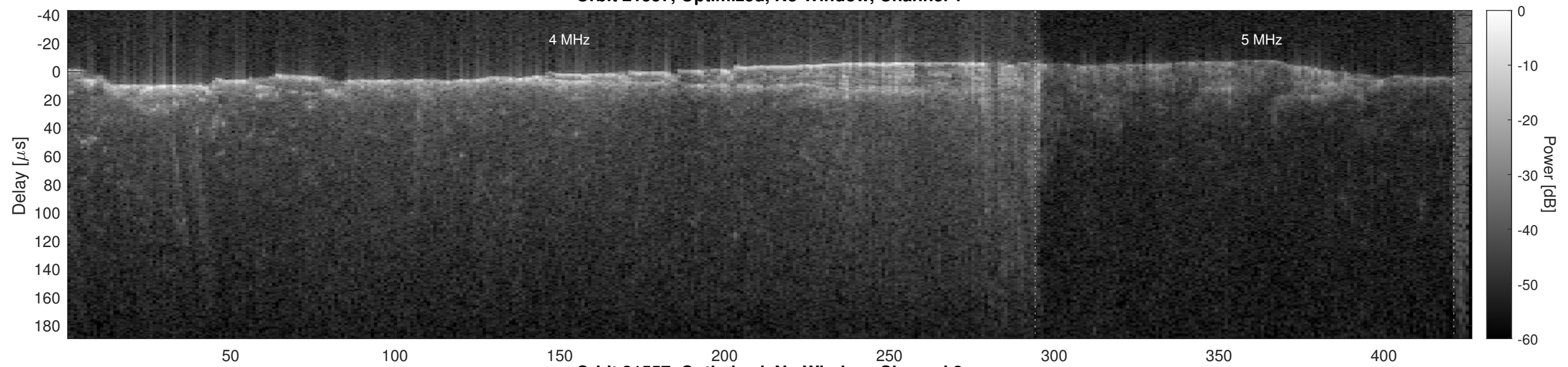
Orbit 21557, Optimized, No Window, Channel 2
