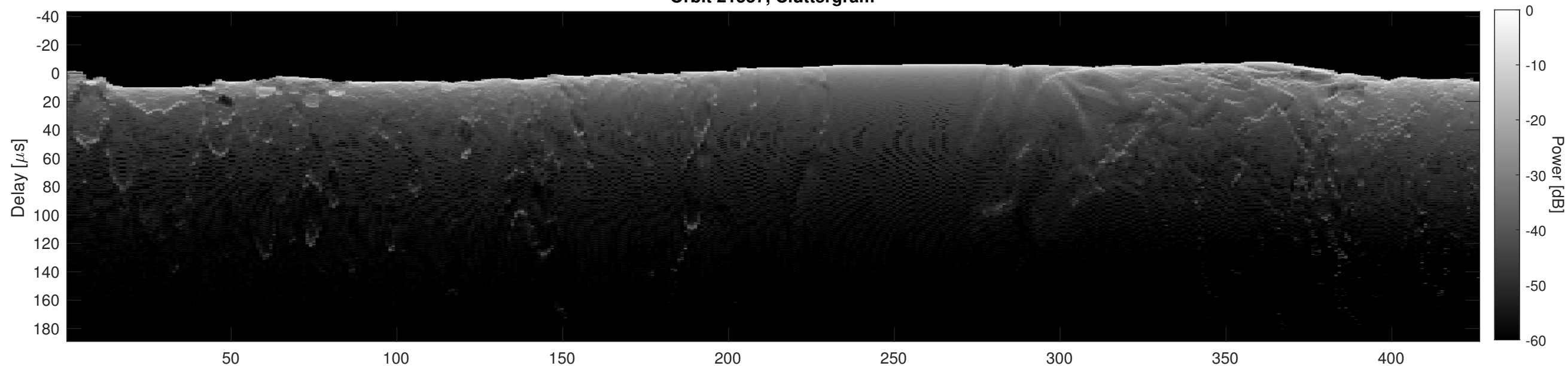
Orbit 21557, Cluttergram
