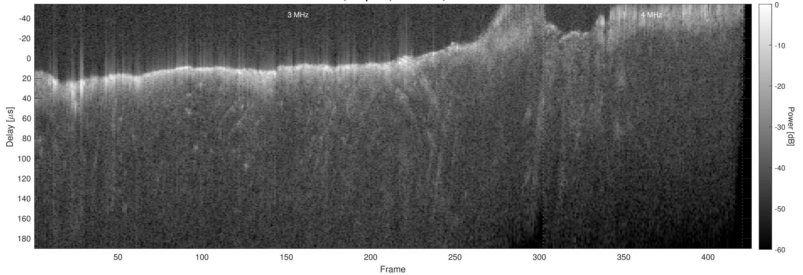
Orbit 21559, Chapman, No Window, Channel 2
