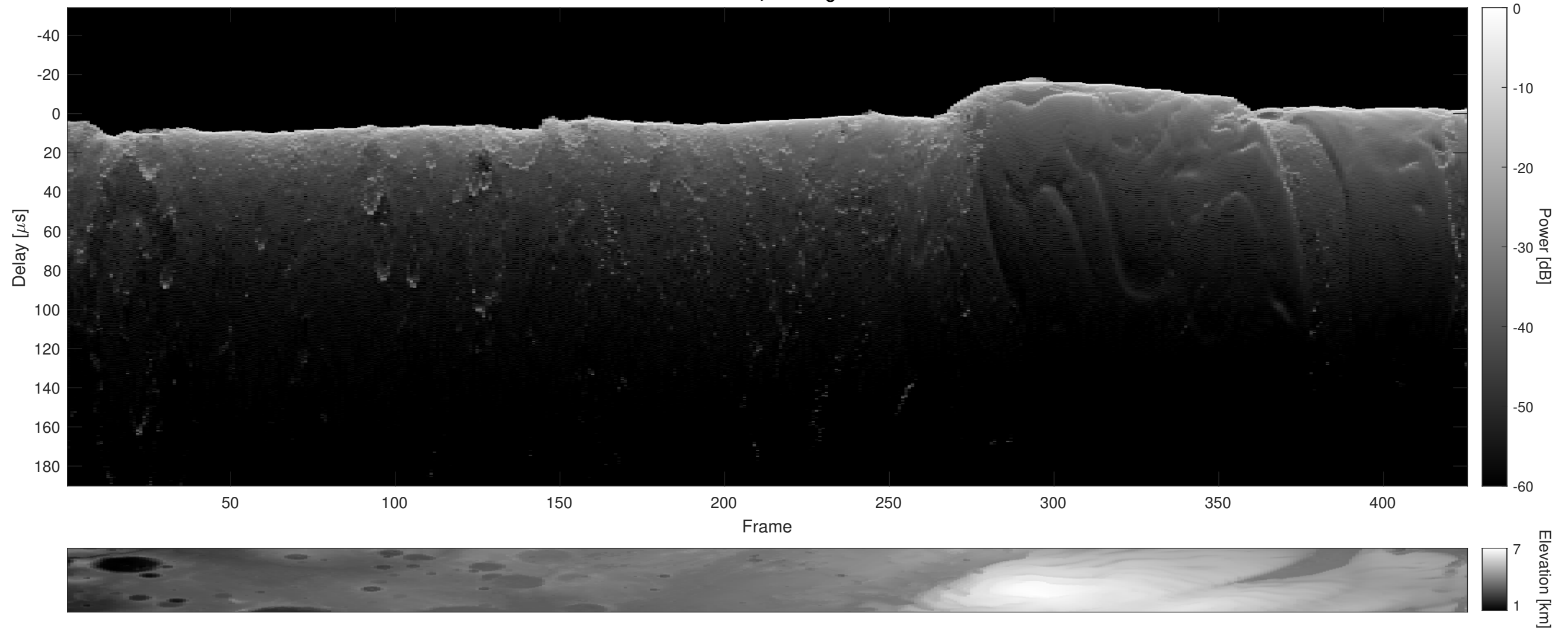
Orbit 21559, Cluttergram
