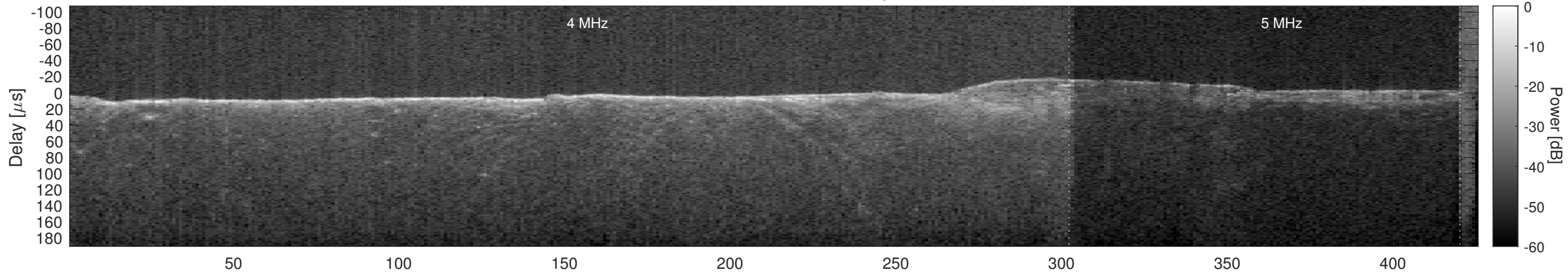
Orbit 21559, Cluttergram
