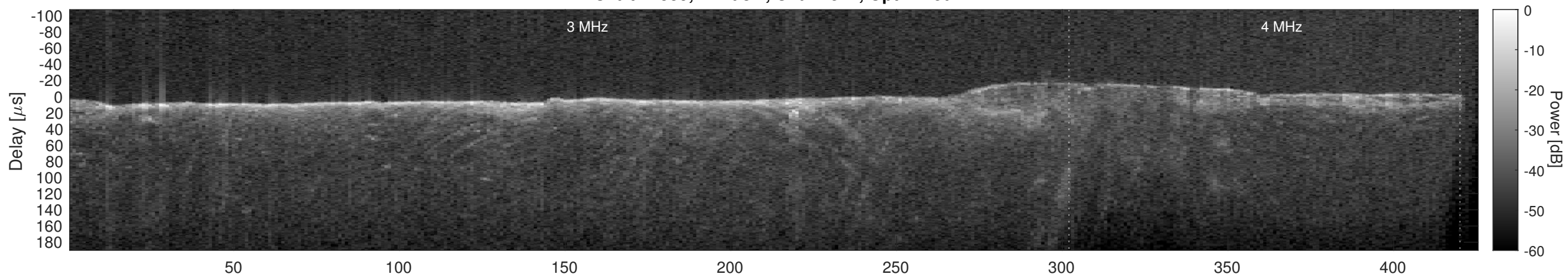
Orbit 21559, Cluttergram
