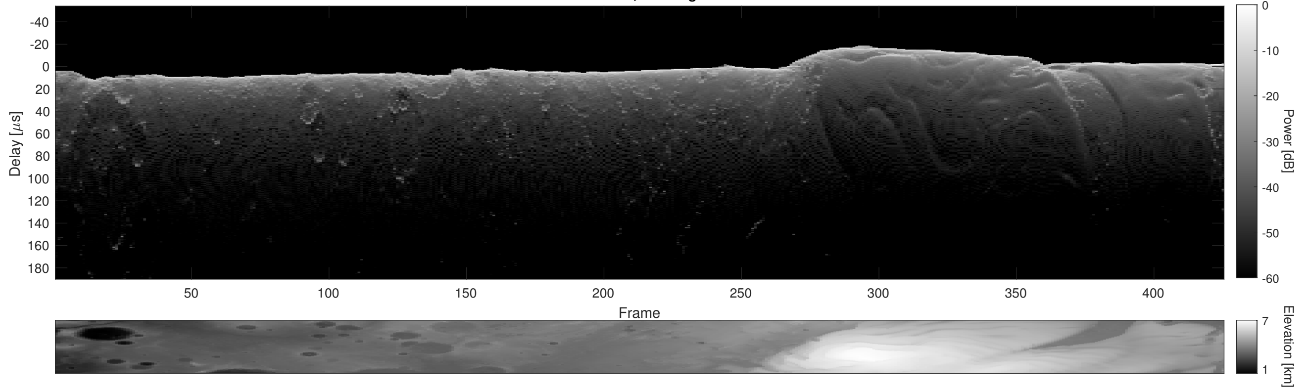
Orbit 21559, Cluttergram
