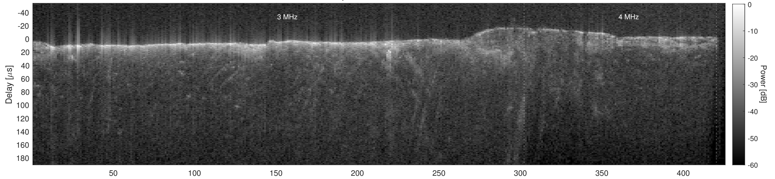
Orbit 21559, Cluttergram
