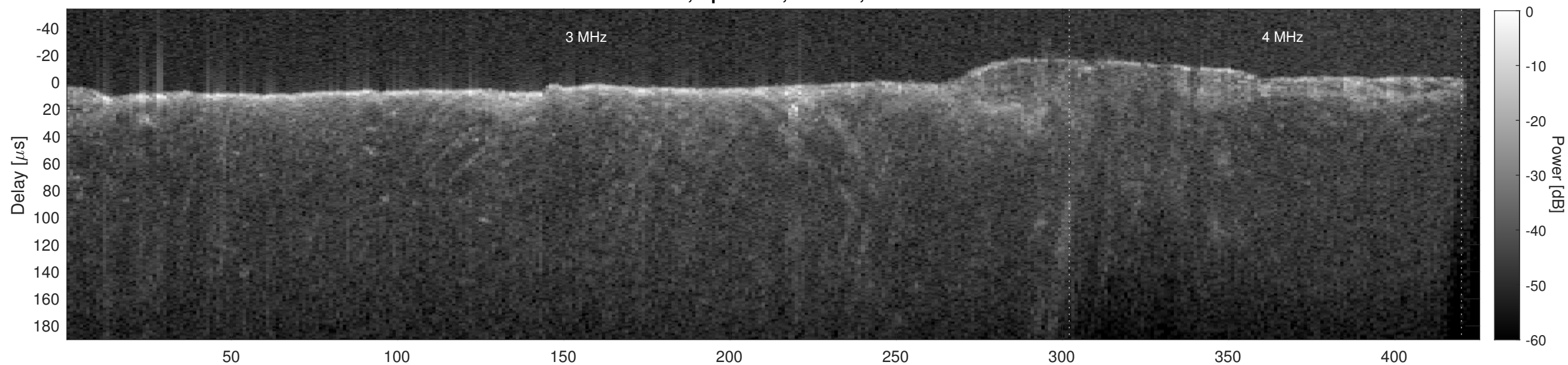
Orbit 21559, Cluttergram
