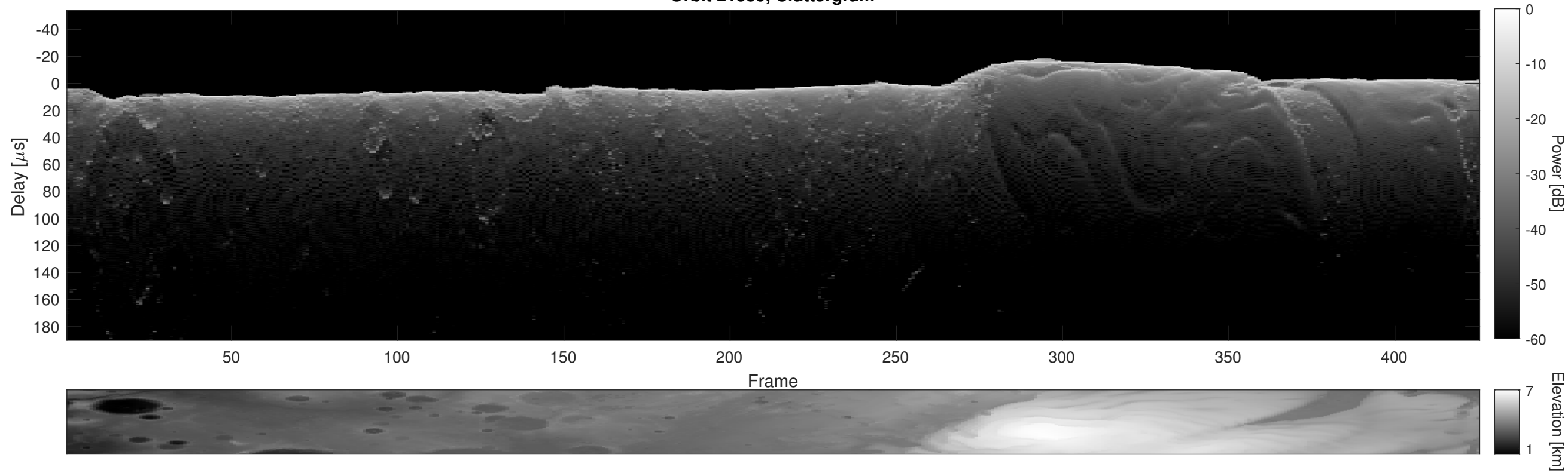
Orbit 21559, Cluttergram
