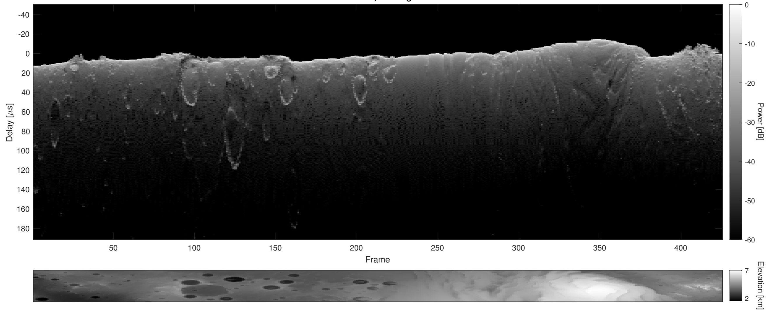
Orbit 21560, Cluttergram
