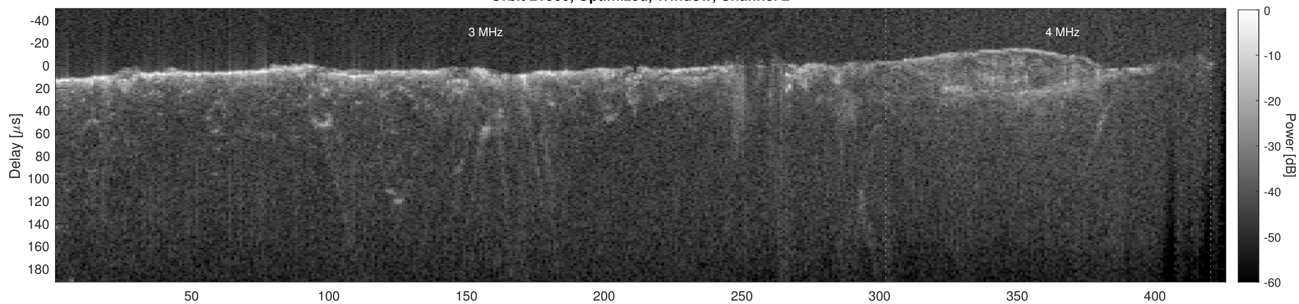
Orbit 21560, Cluttergram
