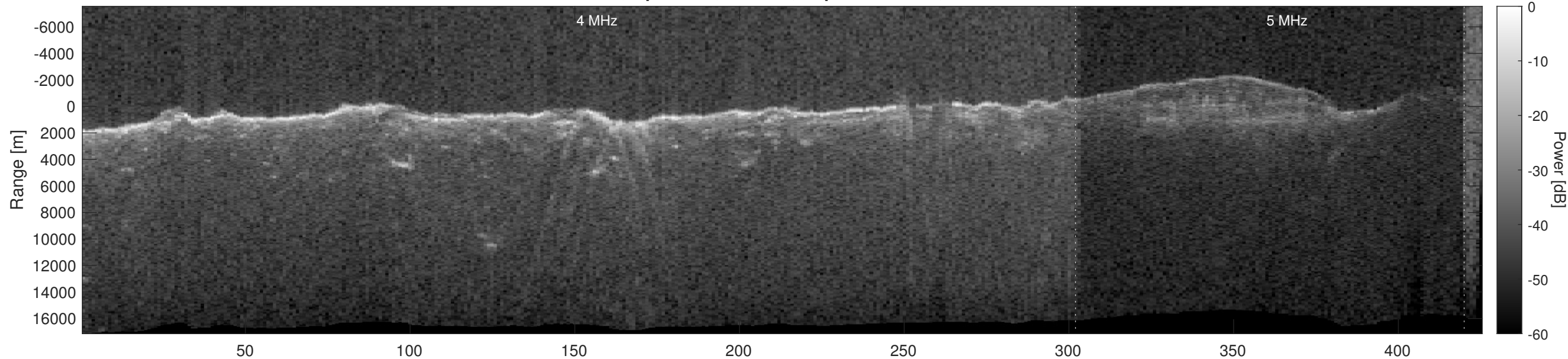
Orbit 21560, Optimized, Window, Depth-Corrected, Channel 2
