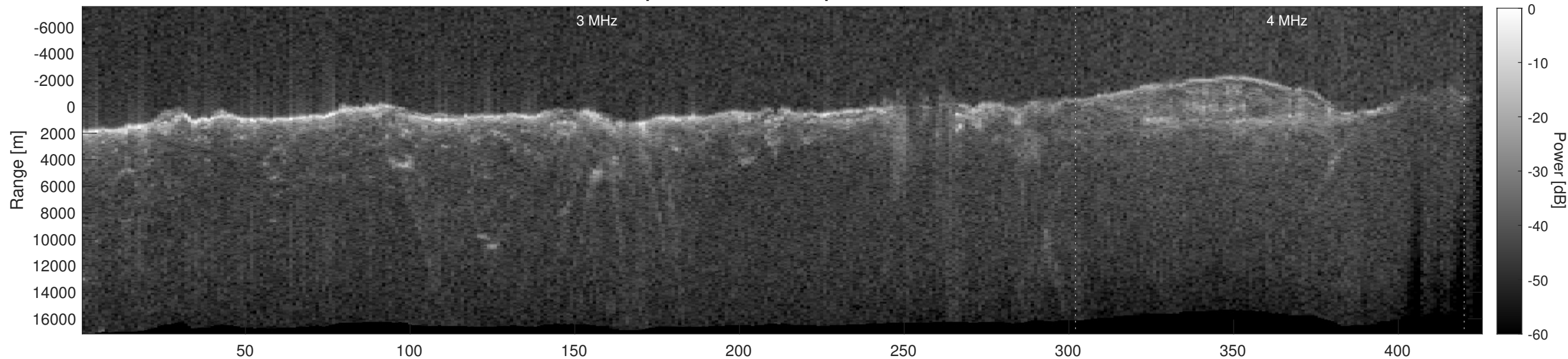
Orbit 21560, Depth-Corrected Cluttergram
