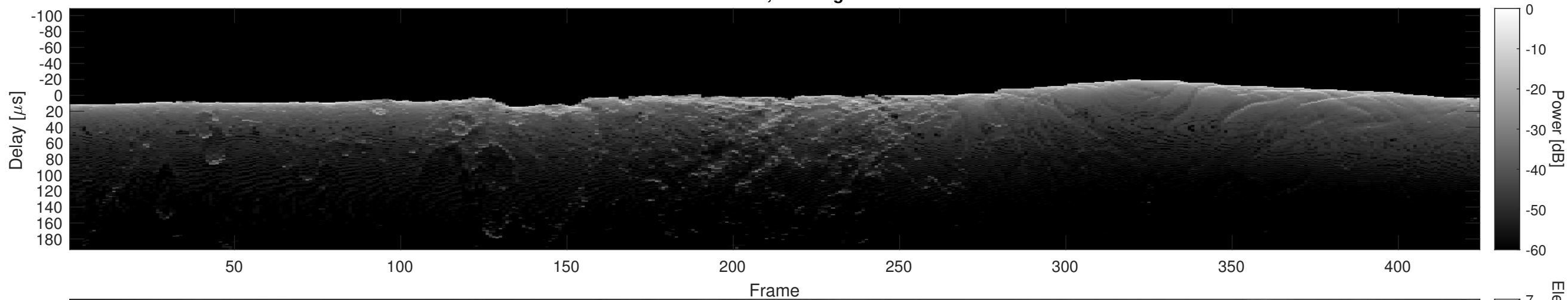
Orbit 21563, Cluttergram
