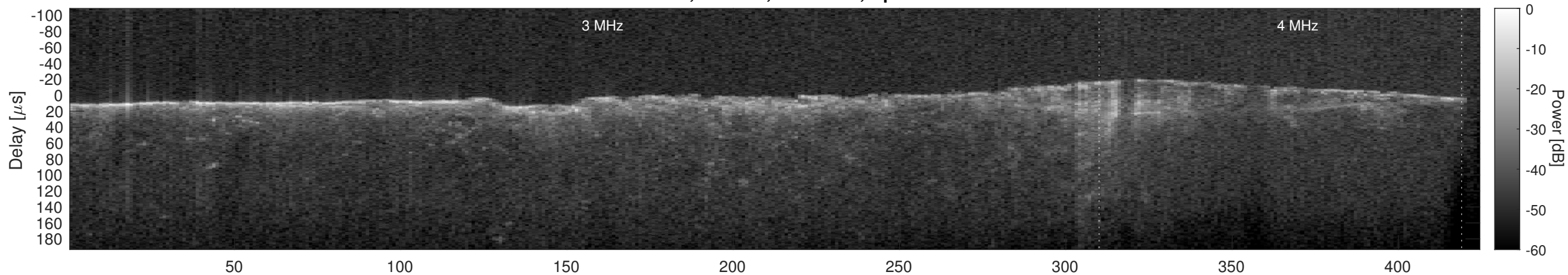
Orbit 21563, Cluttergram
