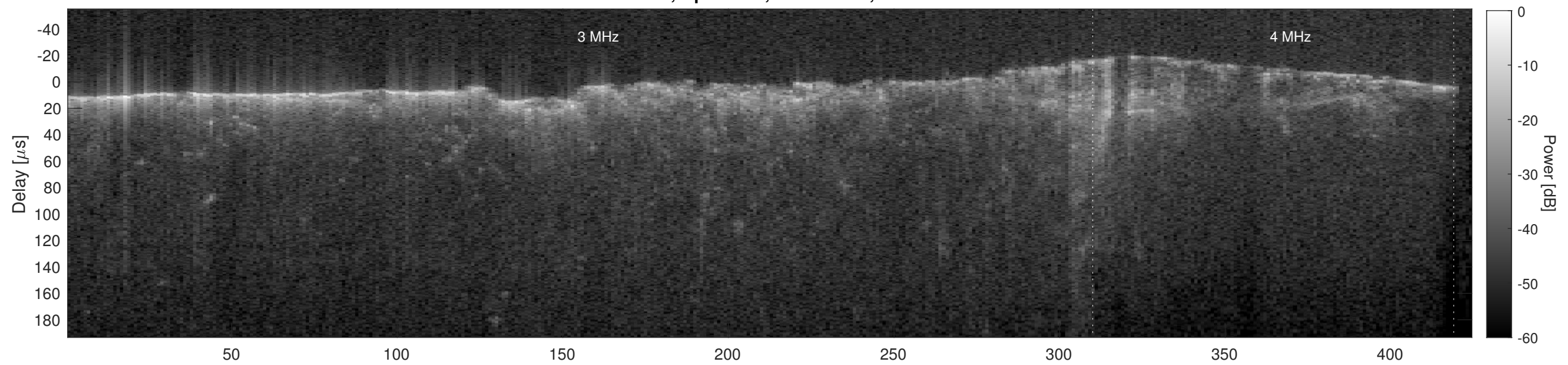
Orbit 21563, Cluttergram
