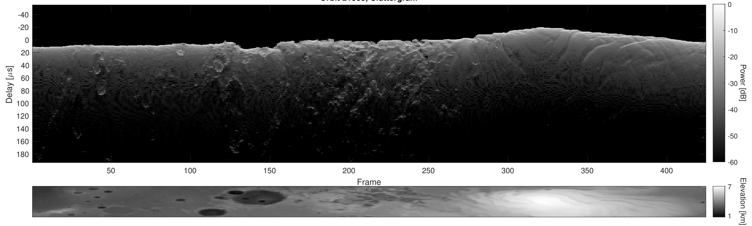
Orbit 21563, Cluttergram
