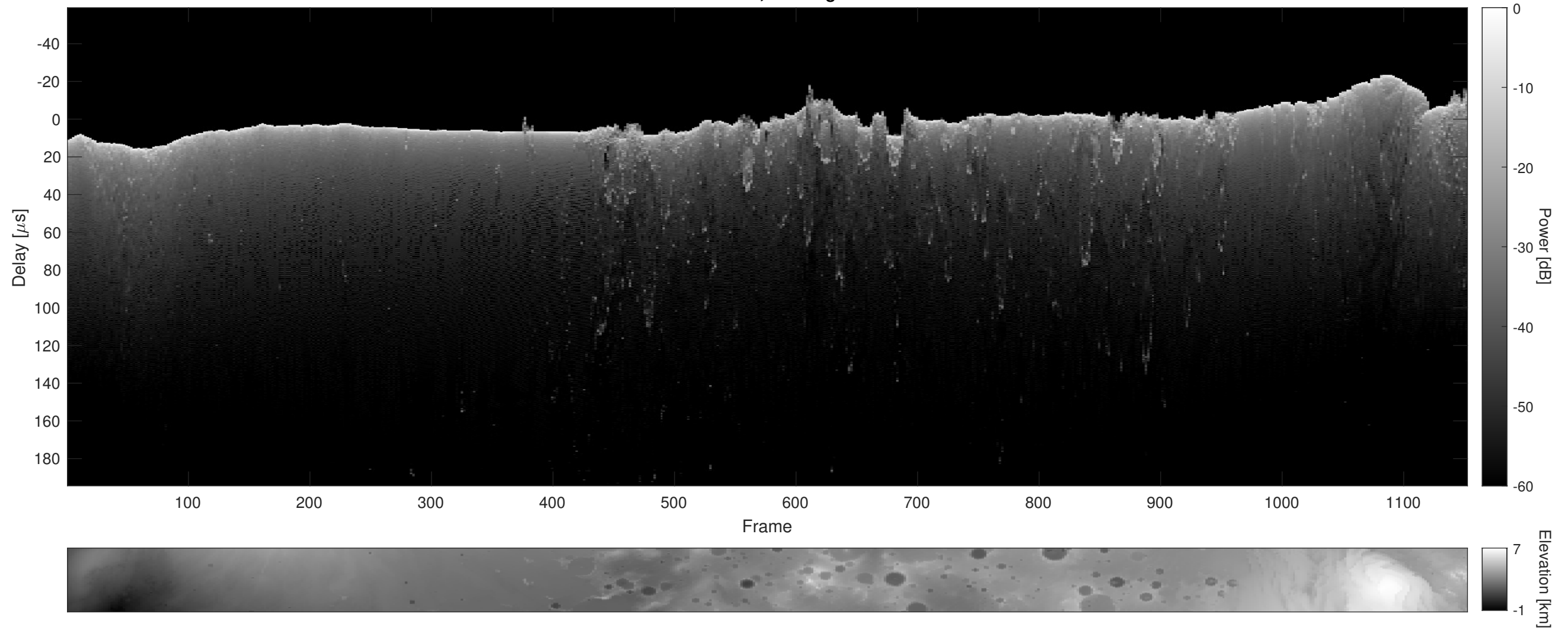
Orbit 21567, Cluttergram
