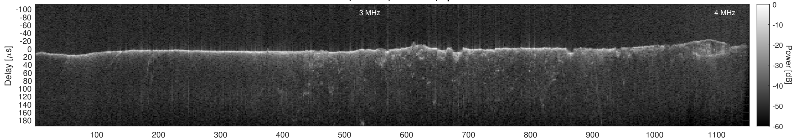
Orbit 21567, Cluttergram
