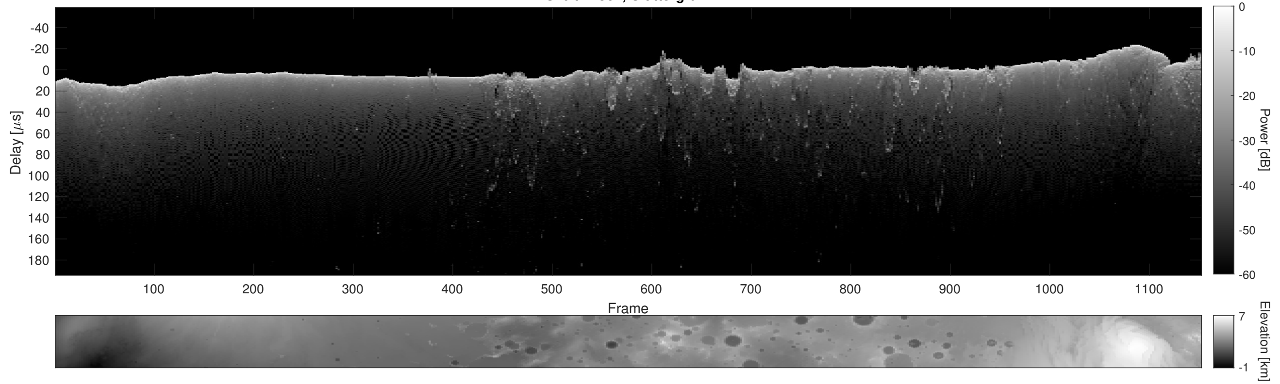
Orbit 21567, Cluttergram
