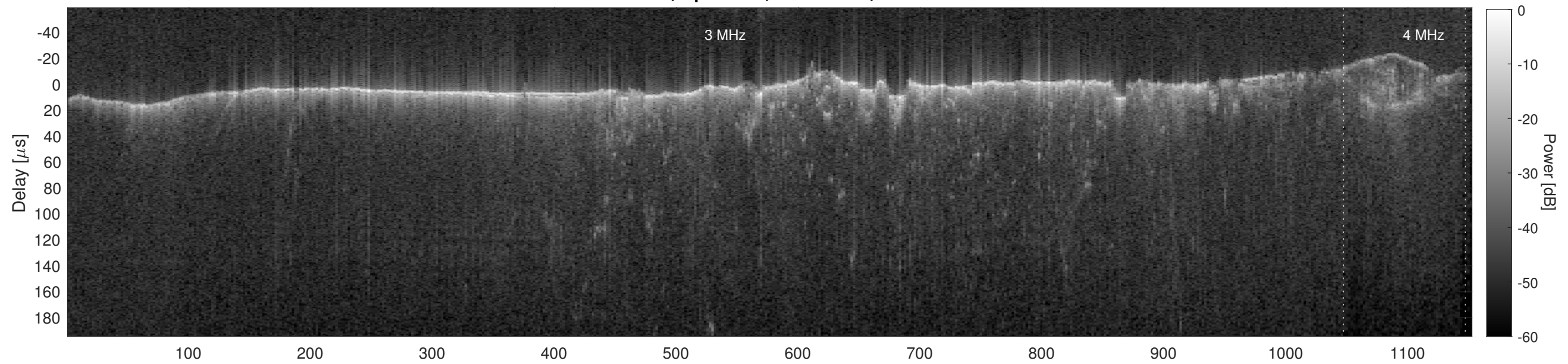
Orbit 21567, Cluttergram
