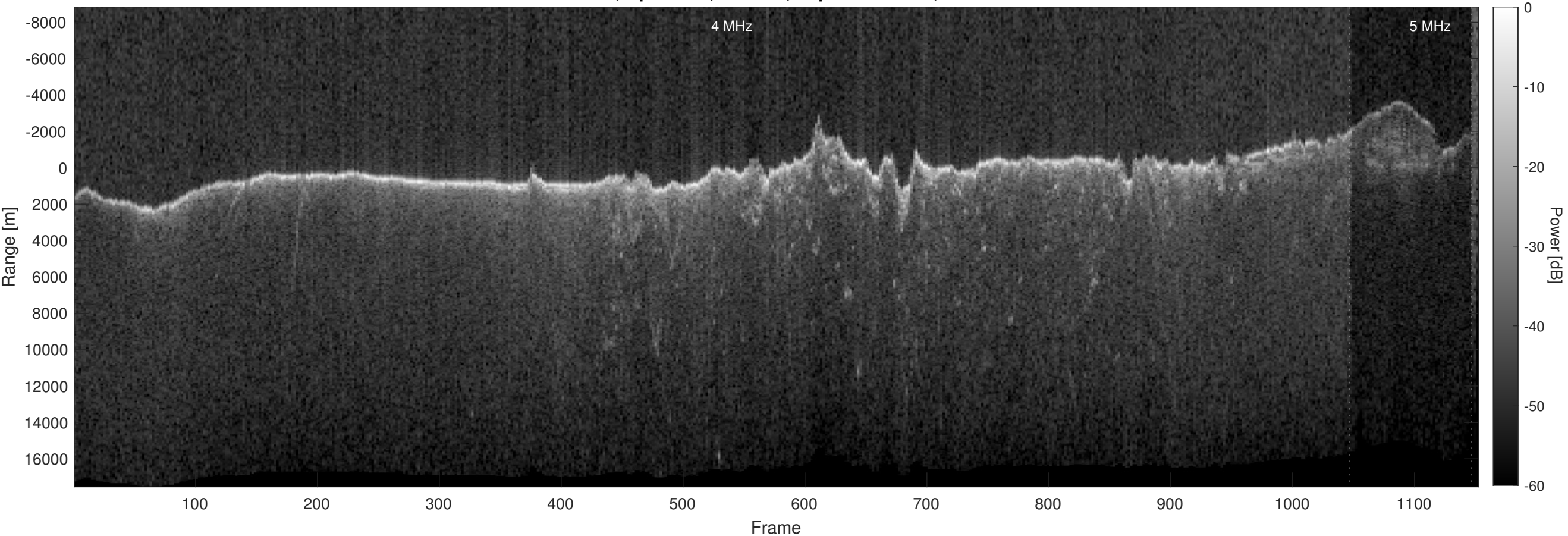
Orbit 21567, Optimized, Window, Depth-Corrected, Channel 2
