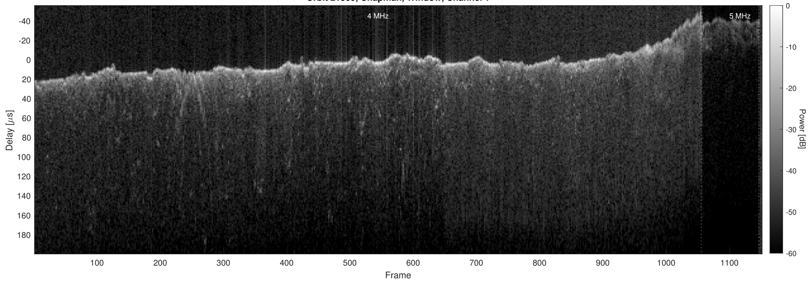
Orbit 21569, Chapman, Window, Channel 2
