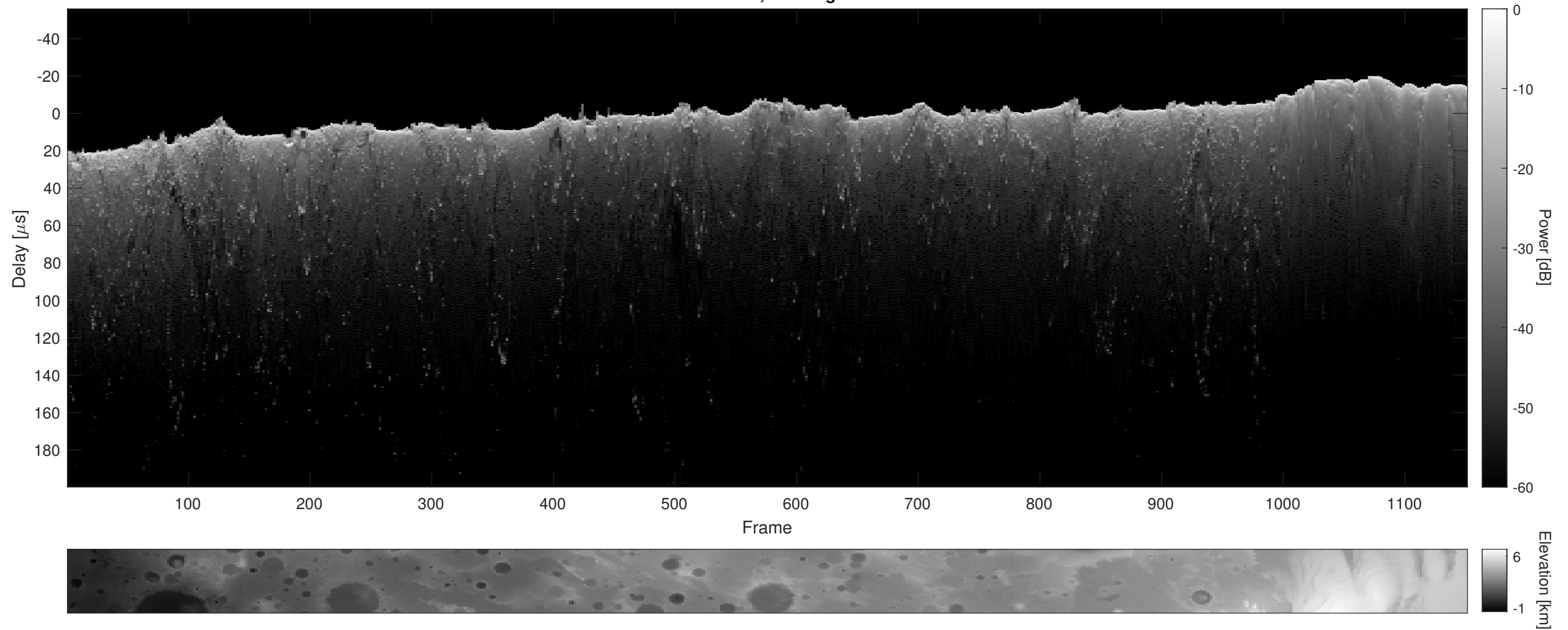
Orbit 21569, Cluttergram
