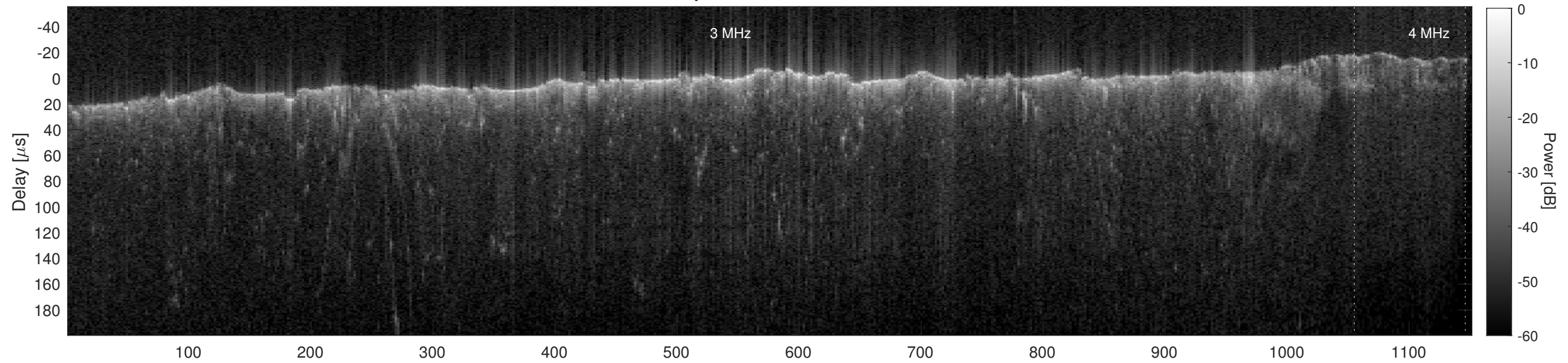
Orbit 21569, Cluttergram
