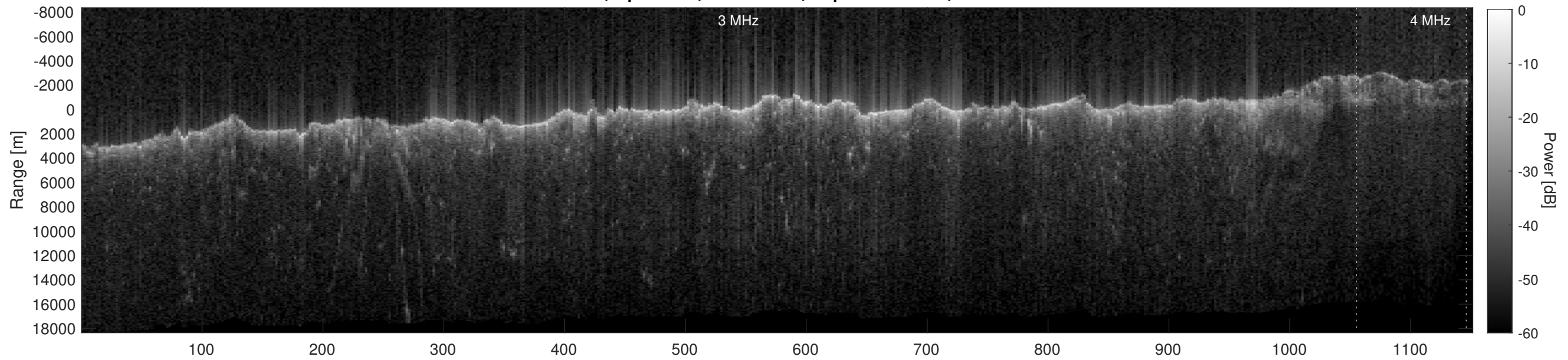
Orbit 21569, Depth-Corrected Cluttergram
