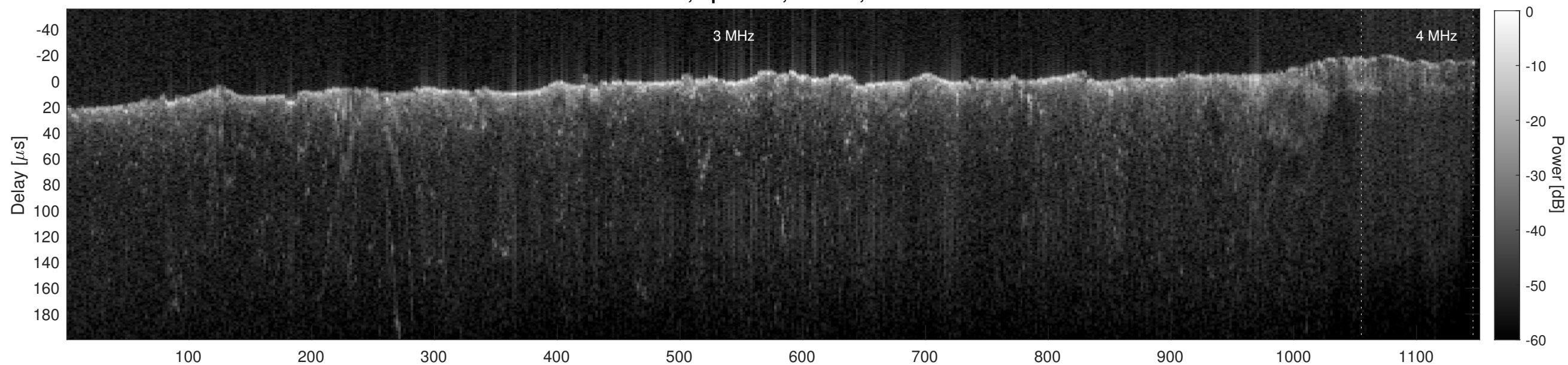
Orbit 21569, Cluttergram
