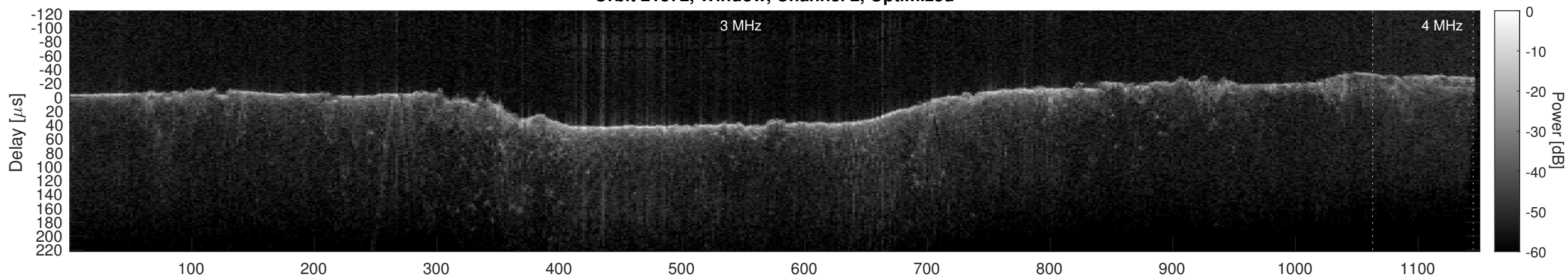
Orbit 21572, Cluttergram
