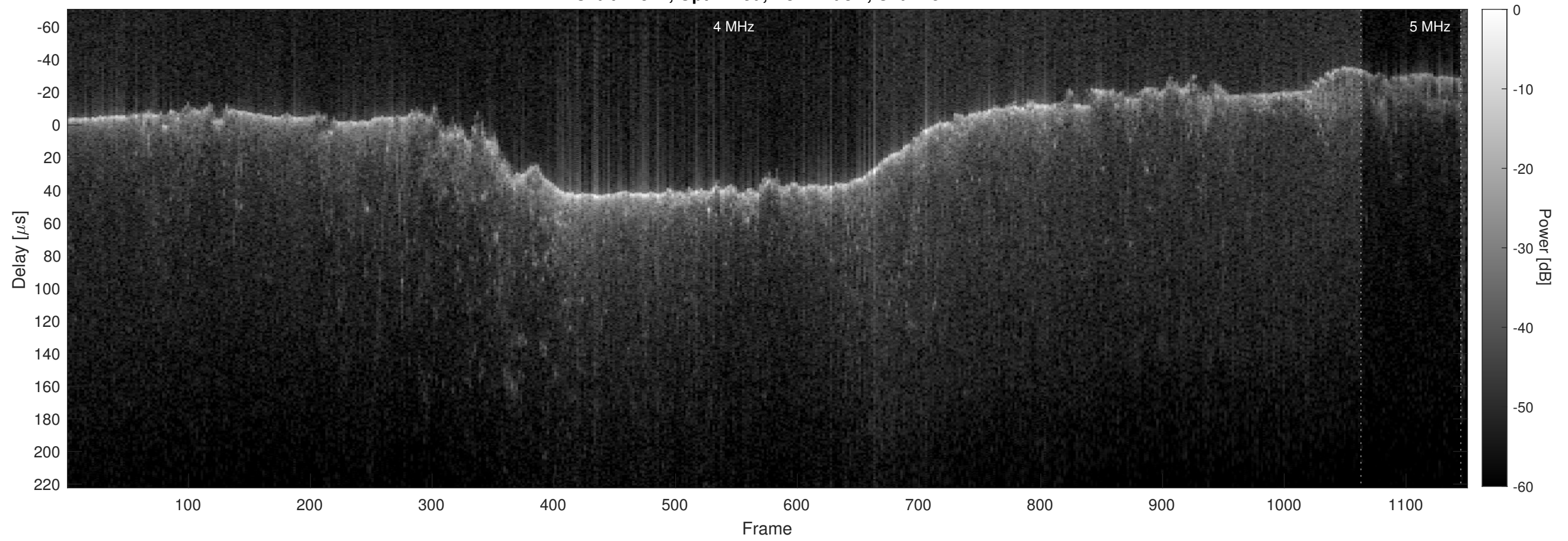
Orbit 21572, Optimized, No Window, Channel 2
