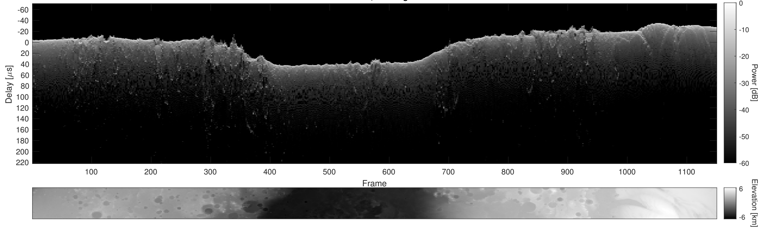
Orbit 21572, Cluttergram
