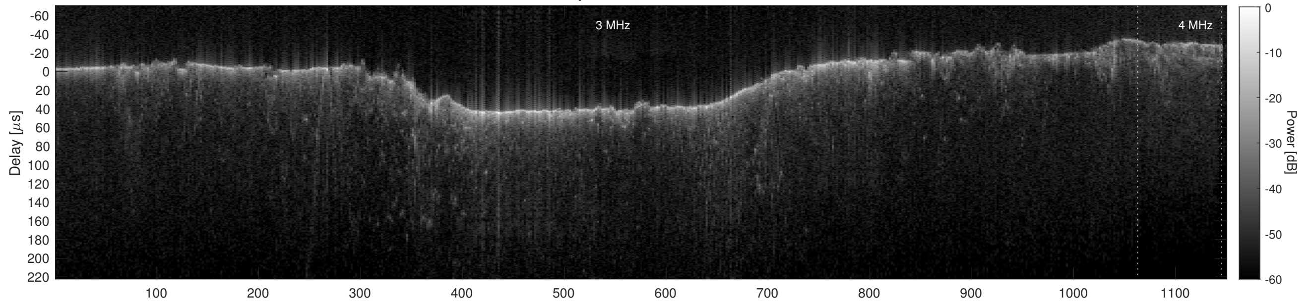
Orbit 21572, Cluttergram
