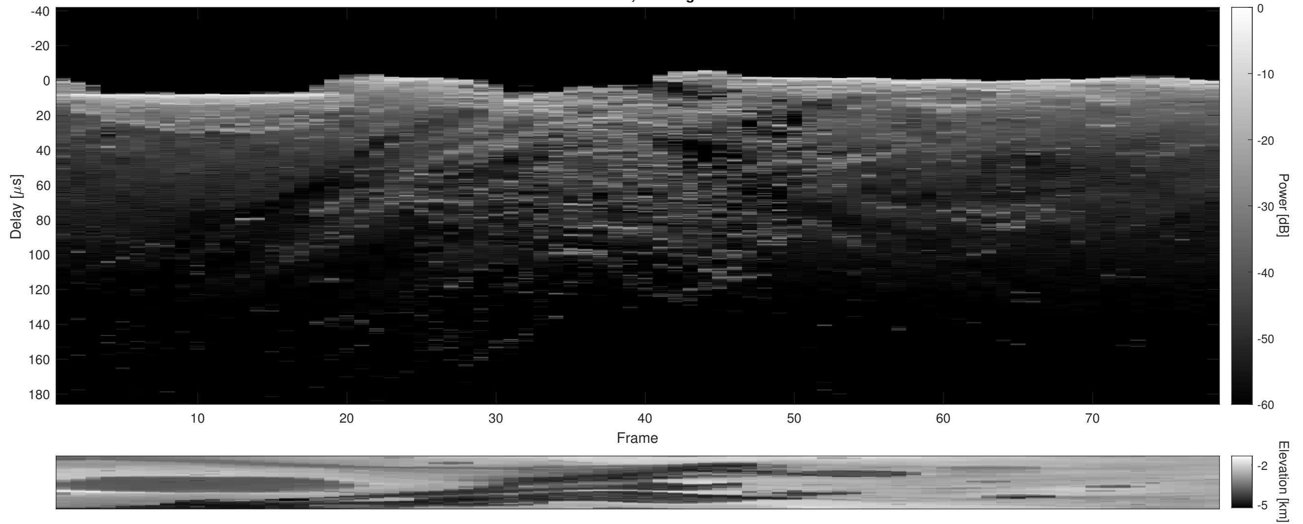
Orbit 21573, Cluttergram
