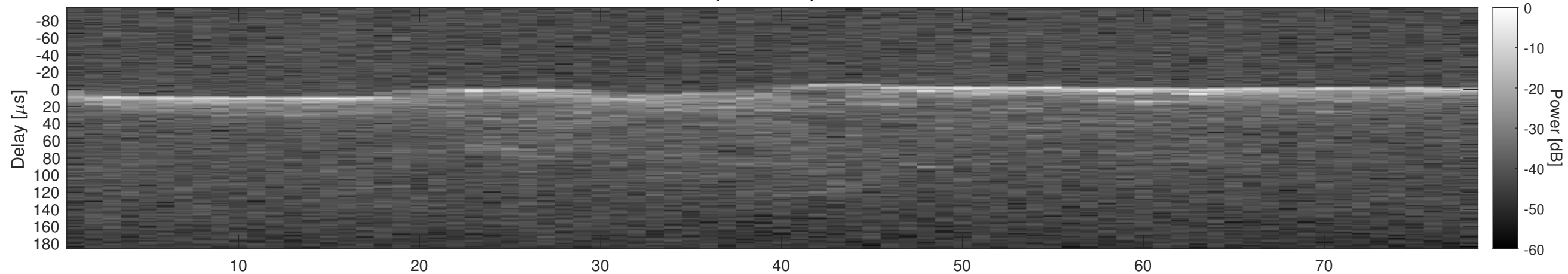
Orbit 21573, Window, Channel 1, Chapman
