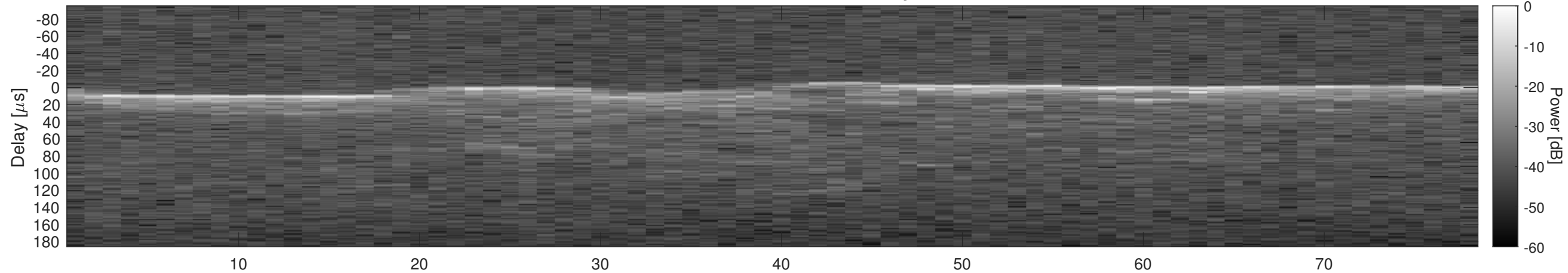
Orbit 21573, Window, Channel 1, Optimized
