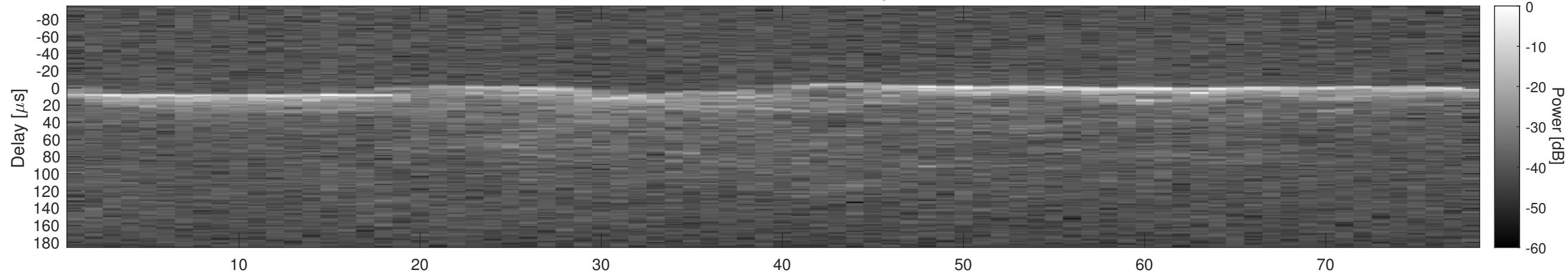
Orbit 21573, Cluttergram
