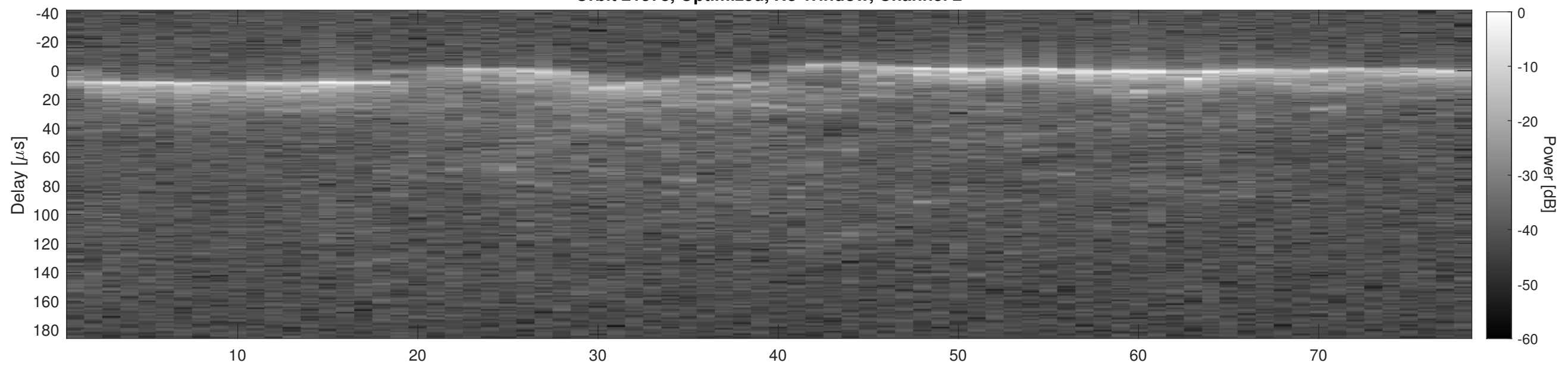
Orbit 21573, Cluttergram
