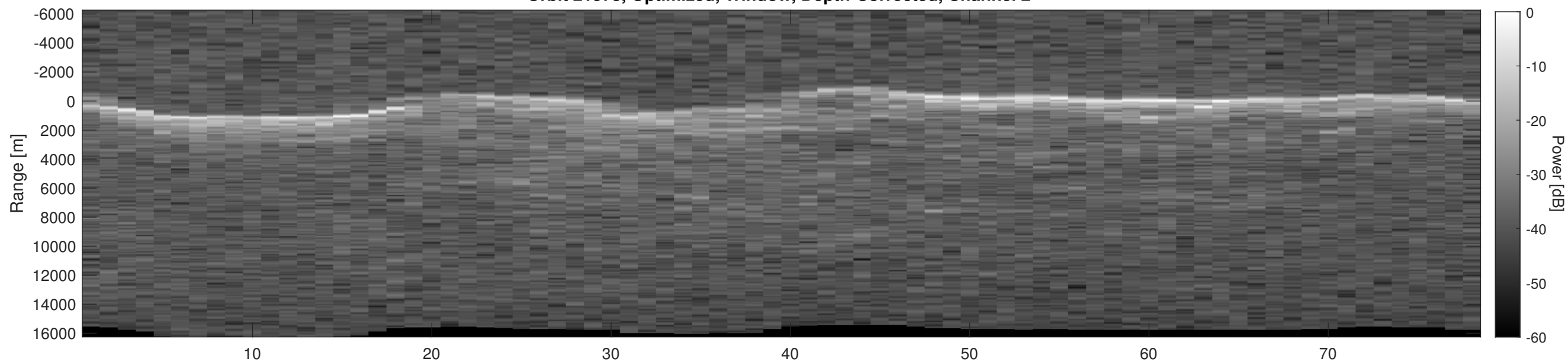
Orbit 21573, Depth-Corrected Cluttergram
