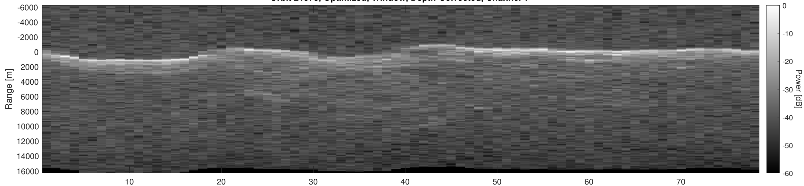
Orbit 21573, Optimized, Window, Depth-Corrected, Channel 2
