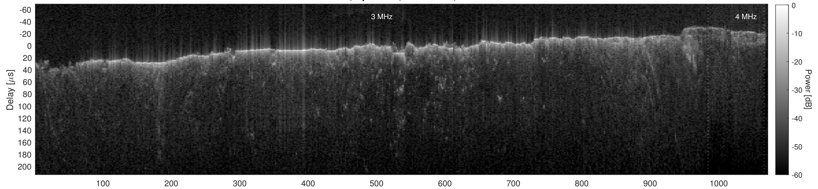
Orbit 21575, Cluttergram
