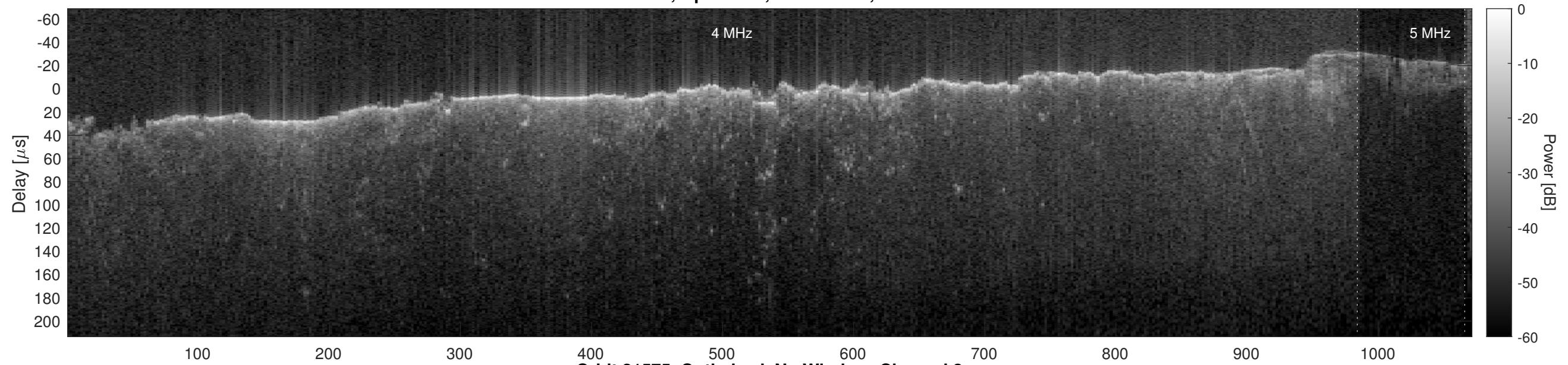
Orbit 21575, Optimized, No Window, Channel 2
