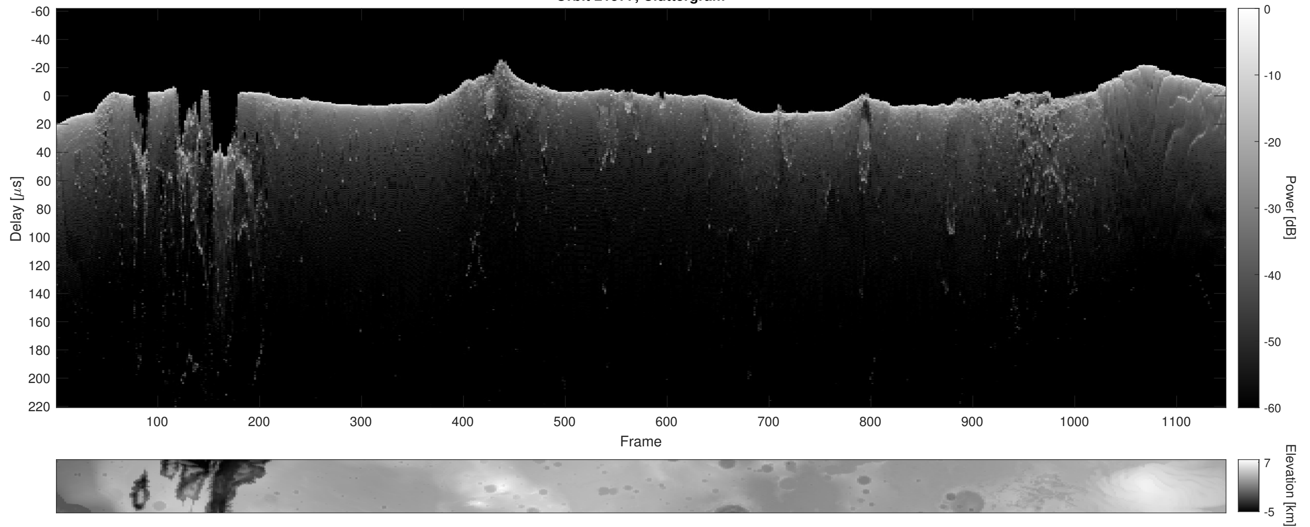
Orbit 21577, Cluttergram
