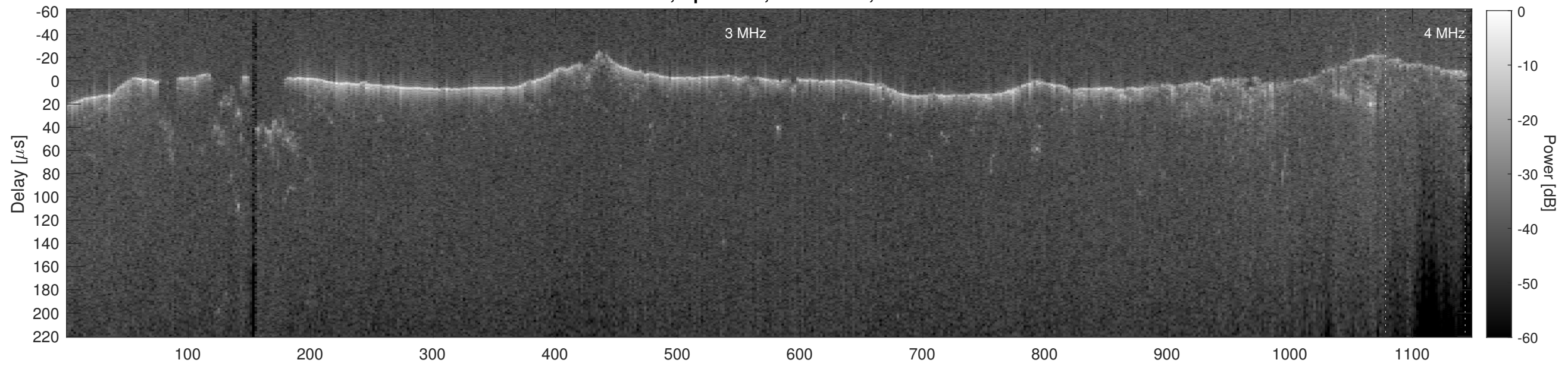
Orbit 21577, Cluttergram
