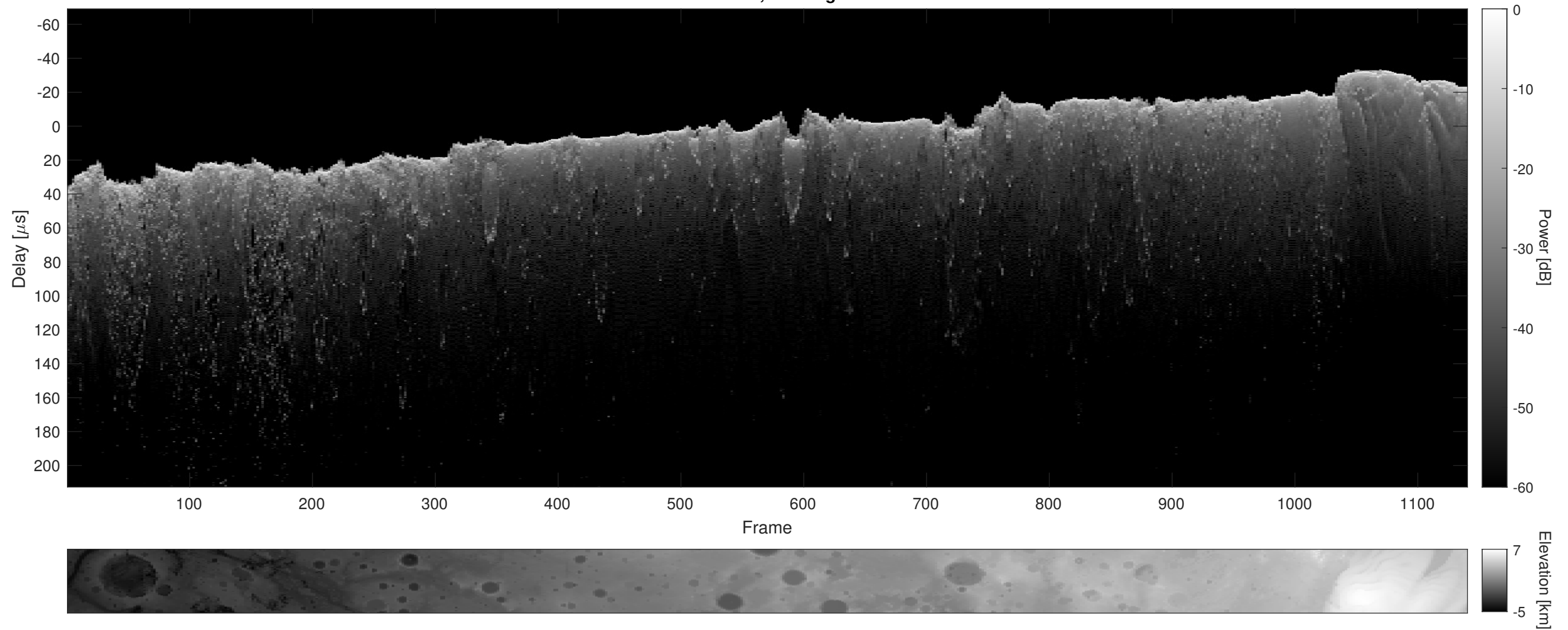
Orbit 21580, Cluttergram
