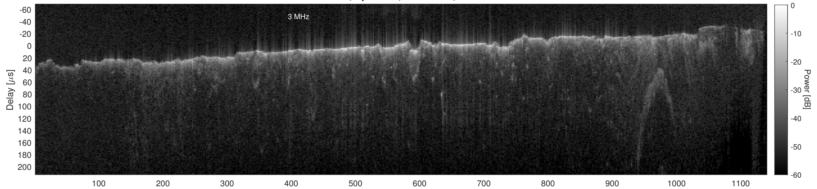
Orbit 21580, Cluttergram
