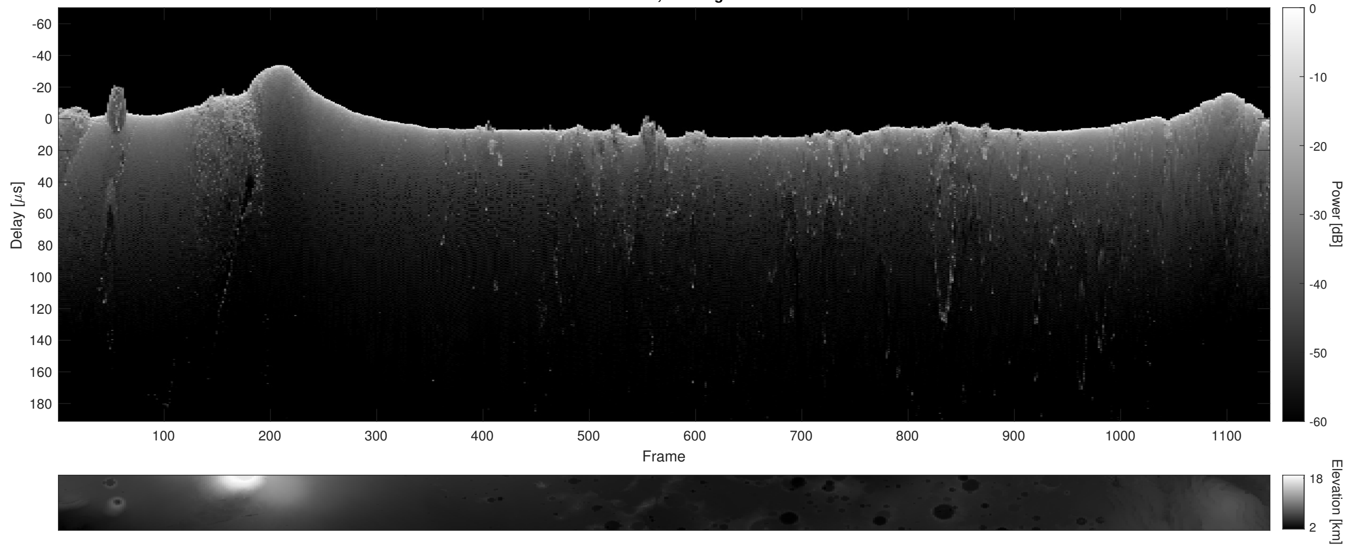
Orbit 21581, Cluttergram
