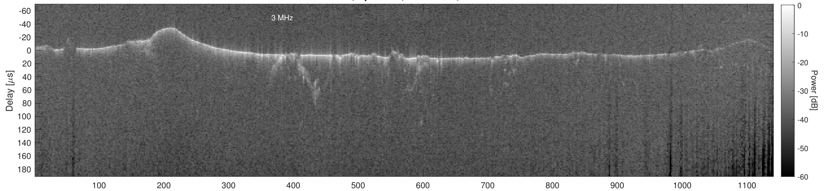
Orbit 21581, Cluttergram
