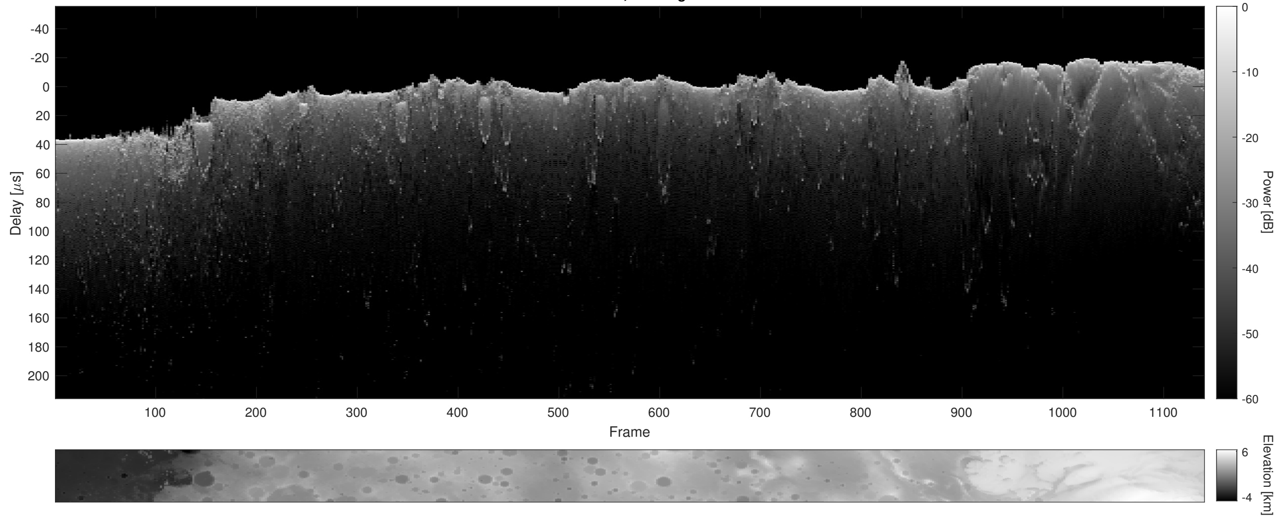
Orbit 21582, Cluttergram
