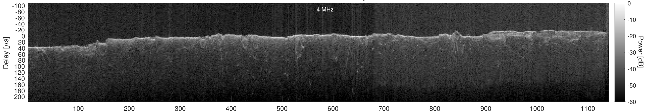
Orbit 21582, Cluttergram
