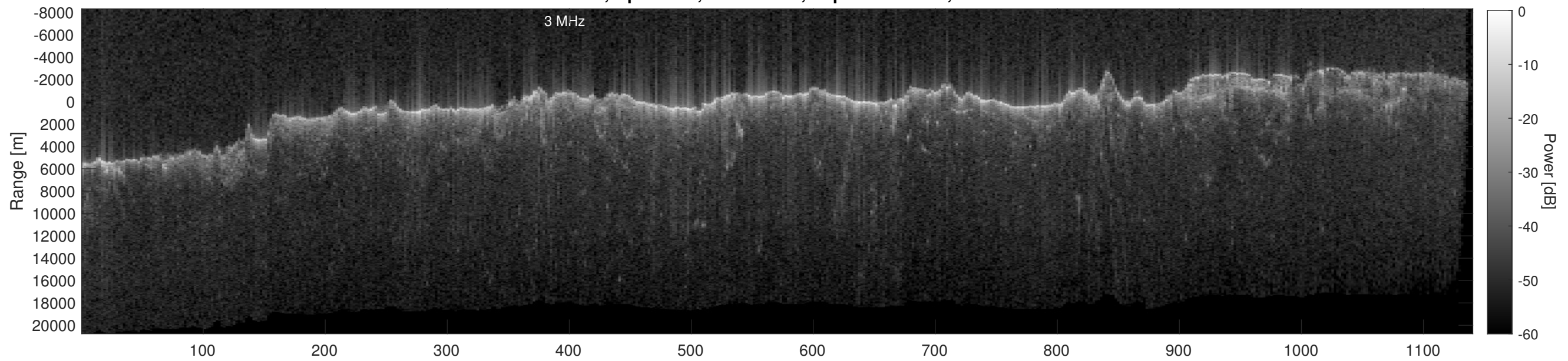
Orbit 21582, Depth-Corrected Cluttergram
