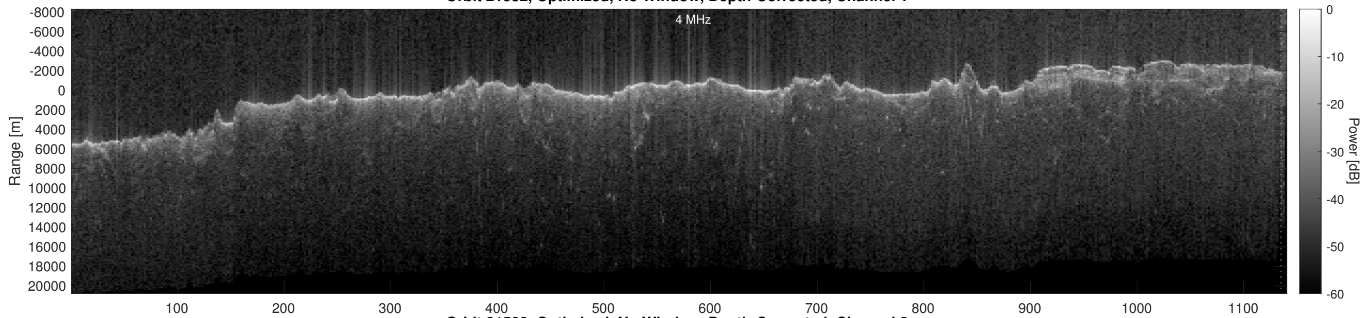
Orbit 21582, Optimized, No Window, Depth-Corrected, Channel 2
