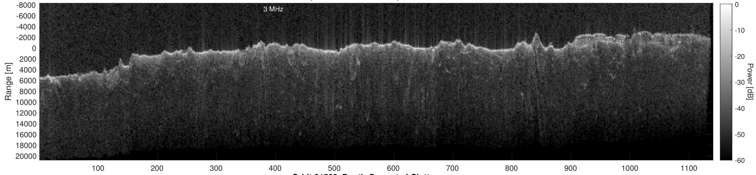
Orbit 21582, Depth-Corrected Cluttergram
