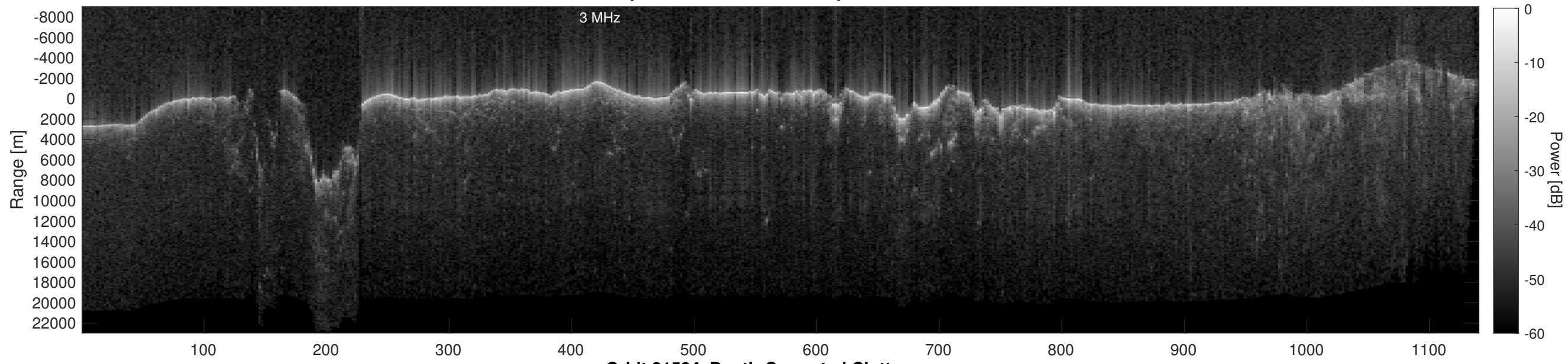
Orbit 21584, Depth-Corrected Cluttergram
