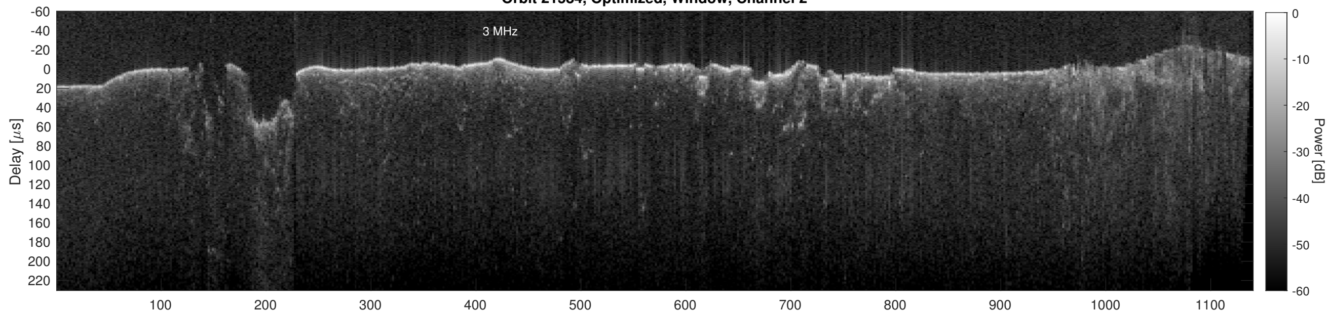
Orbit 21584, Cluttergram
