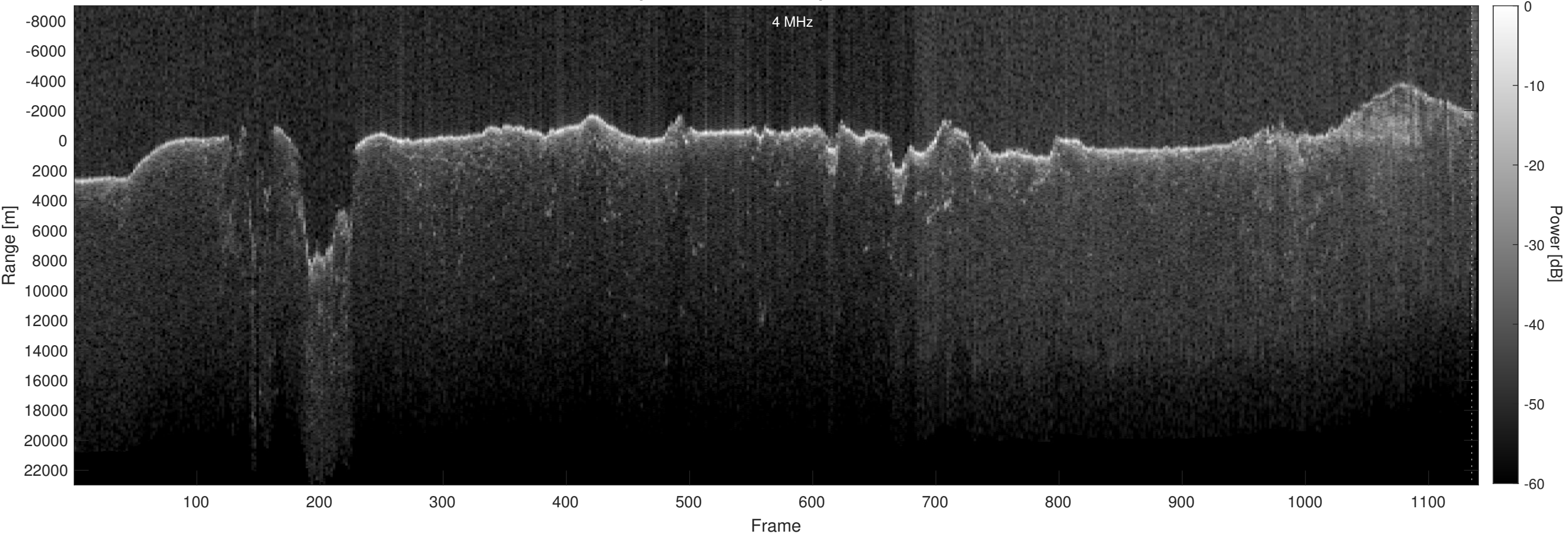
Orbit 21584, Optimized, Window, Depth-Corrected, Channel 2
